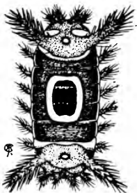
Fig. 416. Saddle-backed slug caterpillar, Sabine stimulea Clemens.
